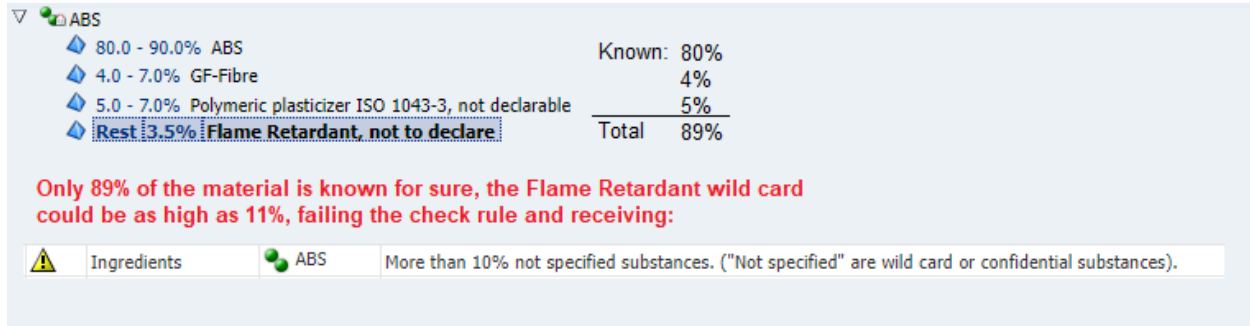
Figure 7 – Use of Portion Type “Rest” for Wildcards Leads to Warning
